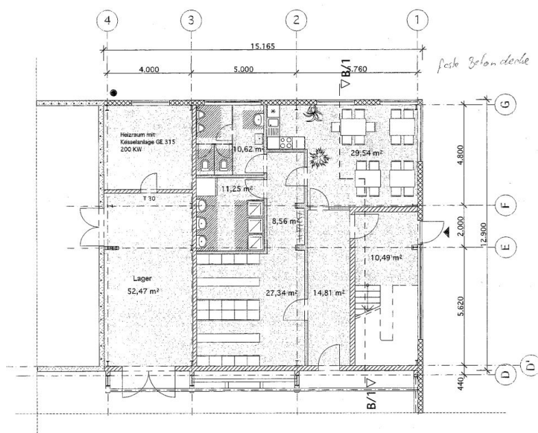
Grundriß Erdgeschoß
