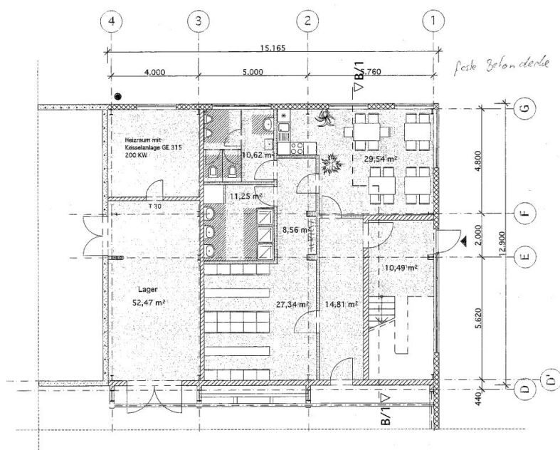
Grundriß Erdgeschoß
