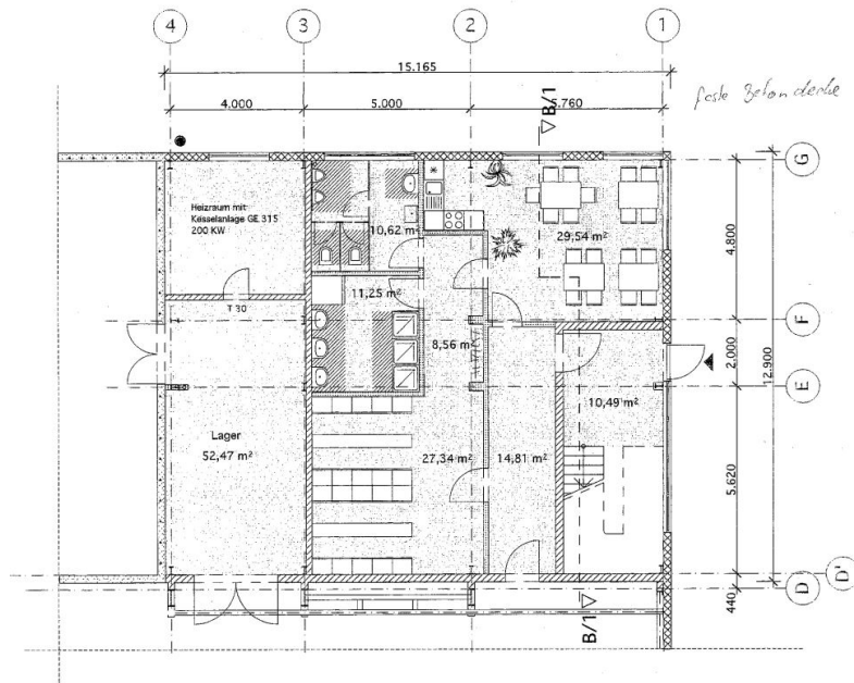
Grundriß Erdgeschoß
