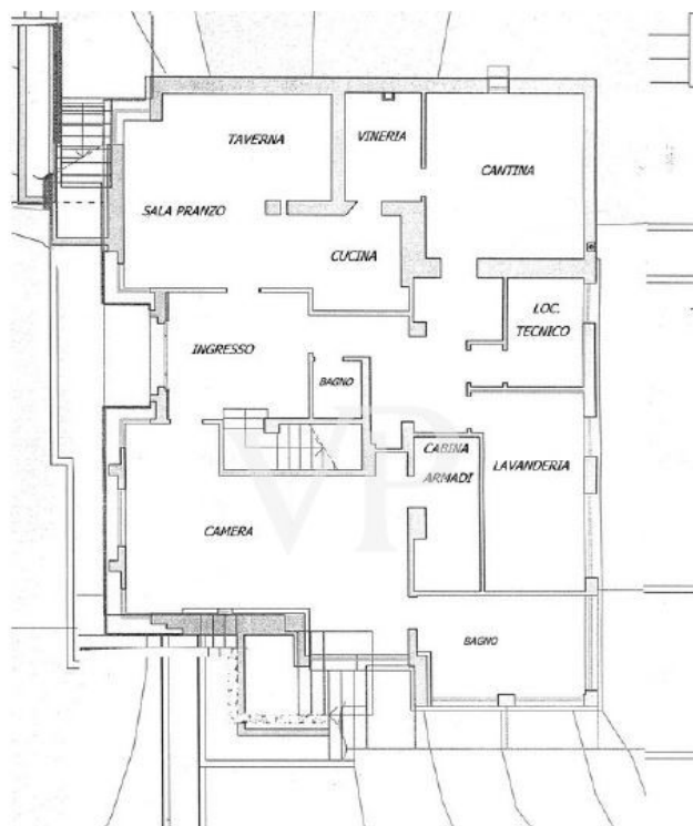
PIANO SEMINTERRATO
