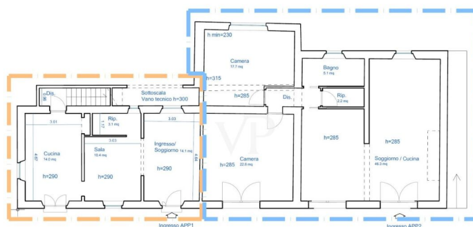
PIANO TERRA
