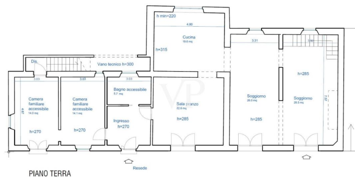
PIANO TERRA
