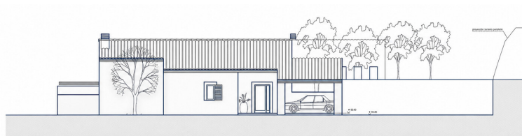
FACHADA PRINCIPAL
