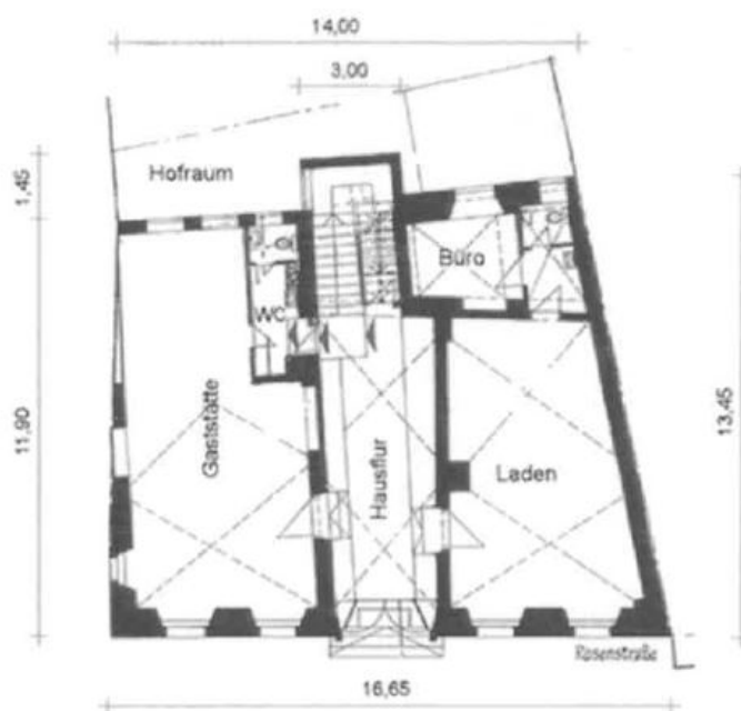
Grundriß Erdgeschoß
